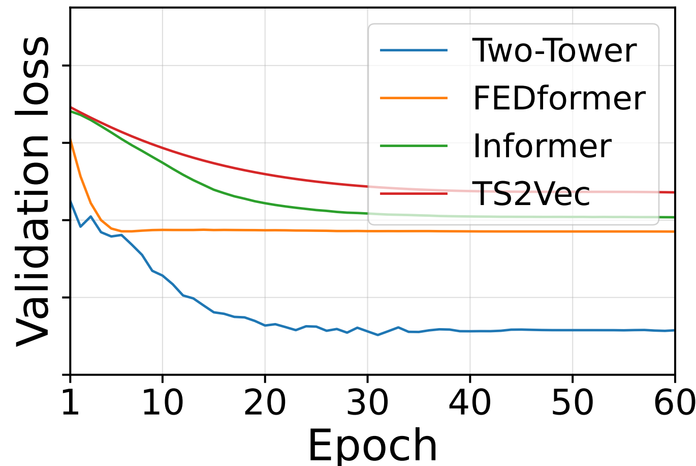
GesturePebbleZ1 — Validation Loss
