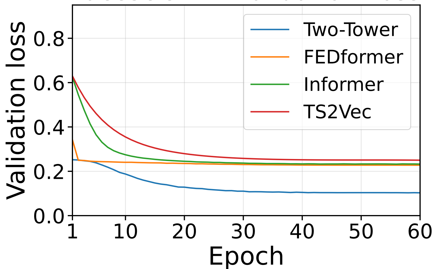
FacesUCR — Validation Loss
