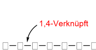
lineare Polysaccharide
