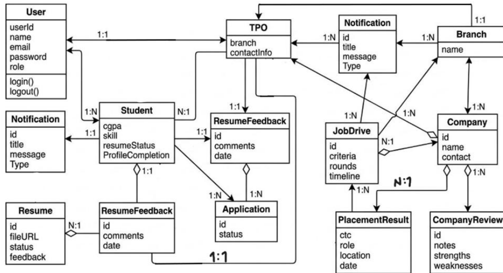
Fig 4.1 Class Diagram
