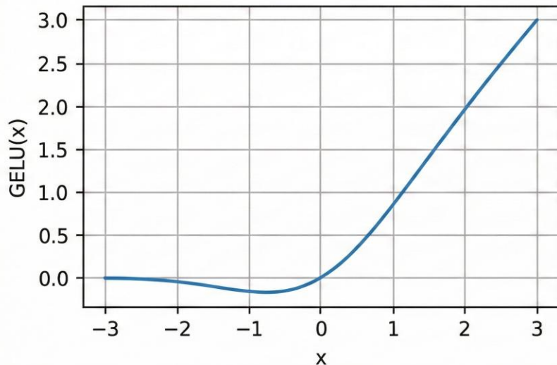
GELU activation function
