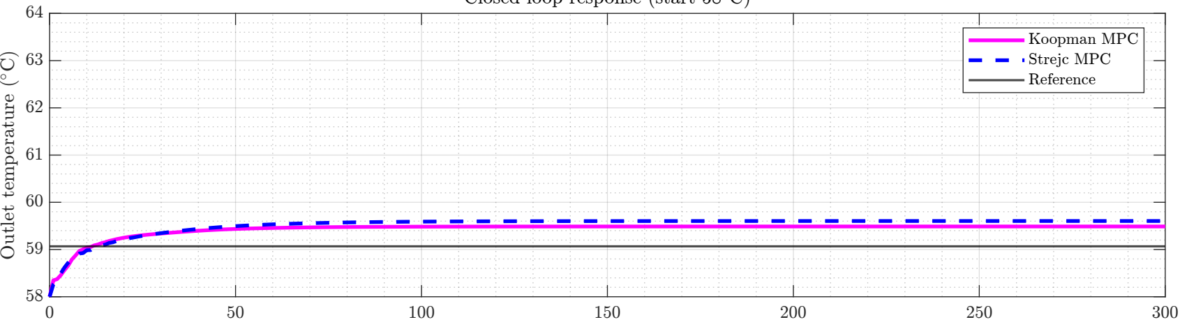
Closed-loop response (start 58°C)
