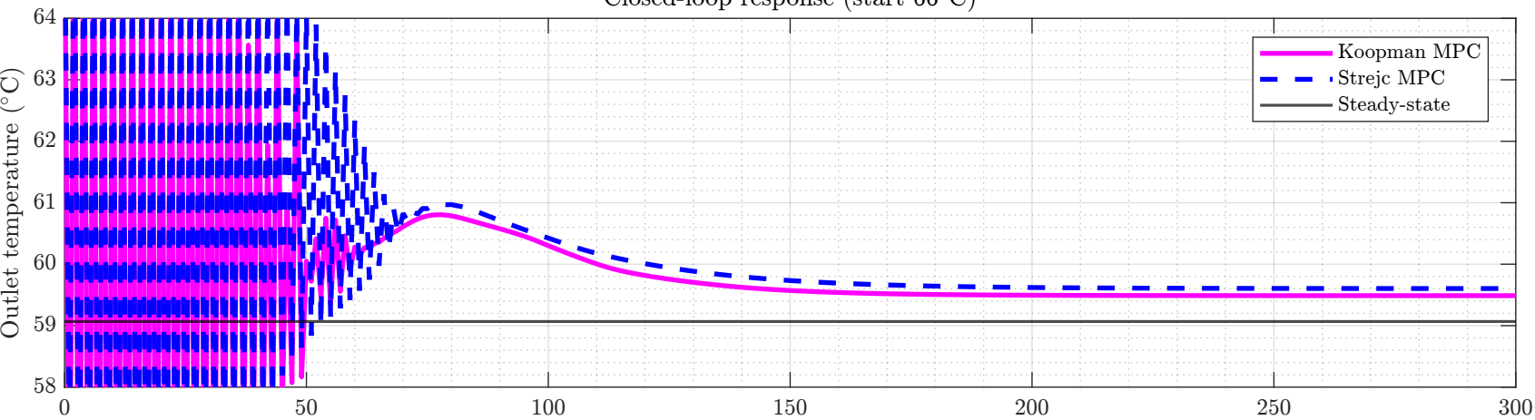
Closed-loop response (start 66°C)
