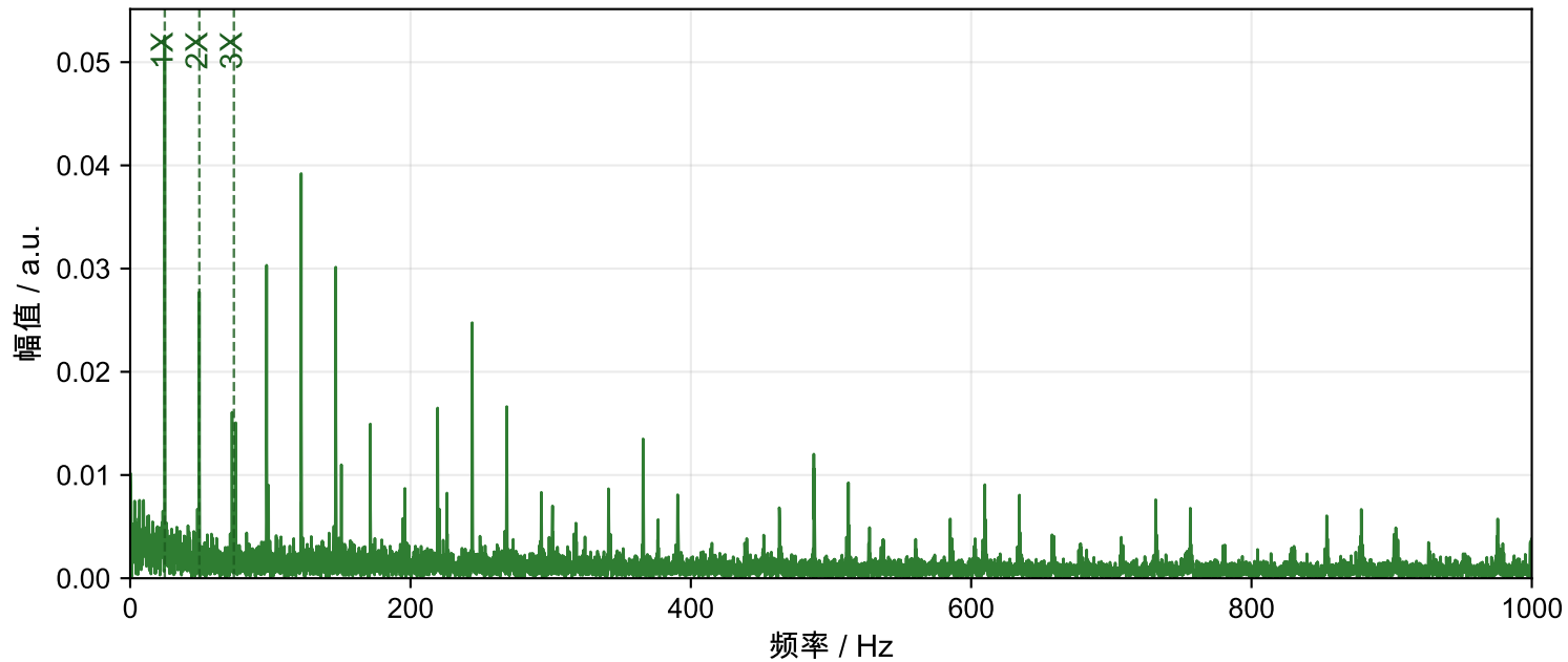
Motor-2 轴承故障 包络谱
