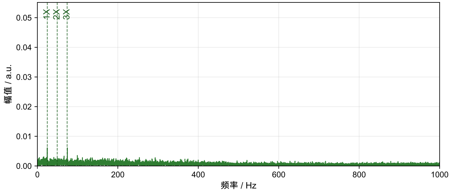
Motor-2 正常 包络谱
