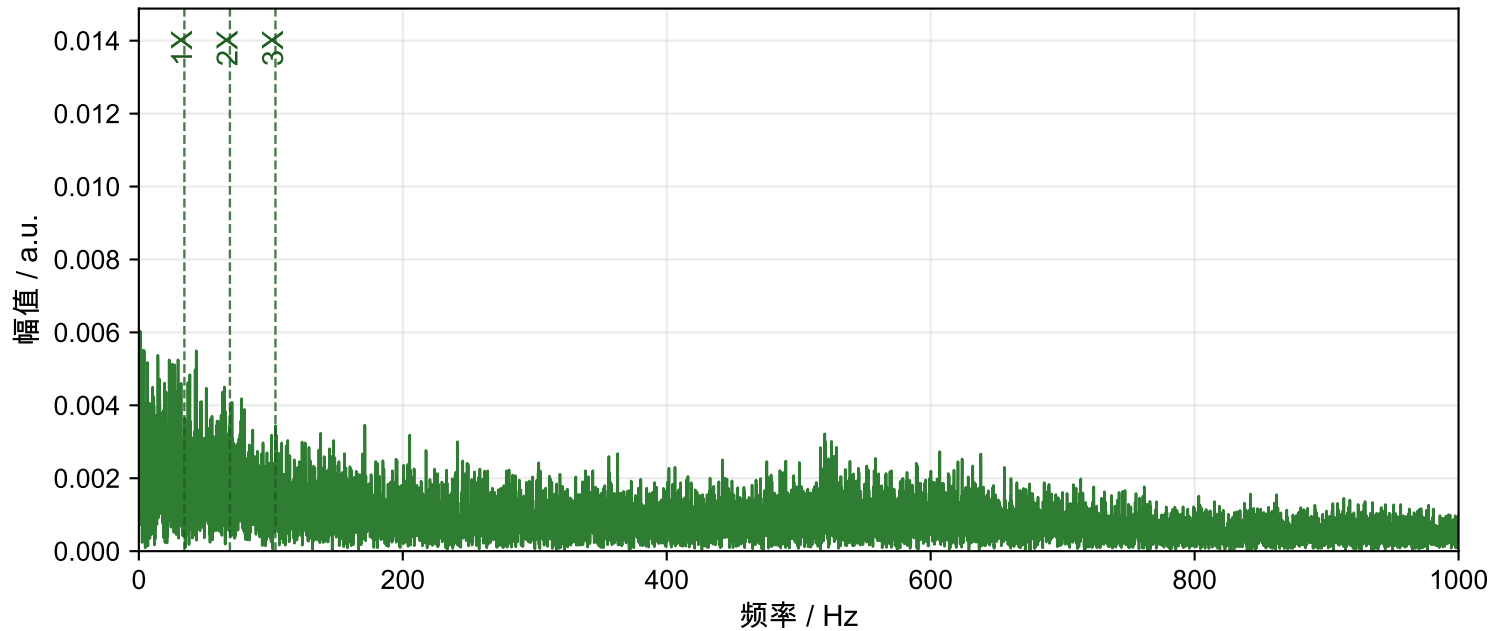
Motor-4 汽蚀 包络谱
