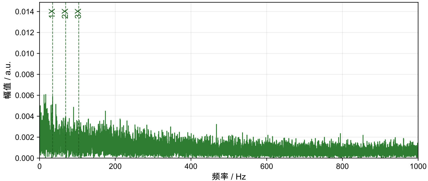
Motor-4 正常 包络谱
