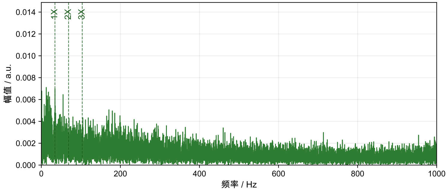
Motor-4 转子不平衡 包络谱
