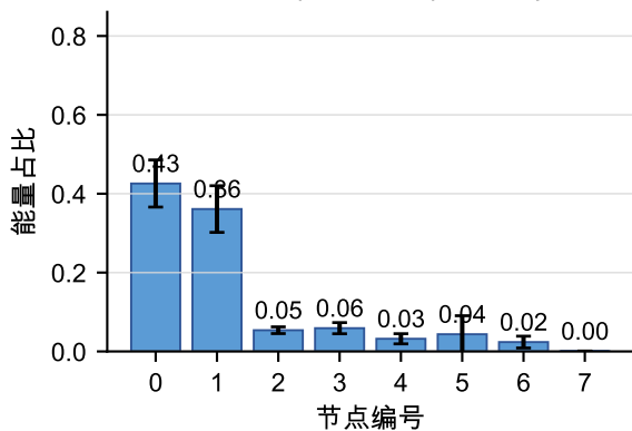
轴承故障 | Motor-2 | 1110 rpm
