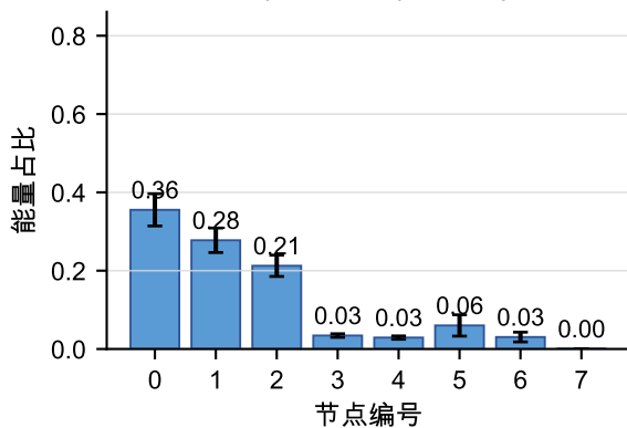
汽蚀 | Motor-4 | 2070 rpm
