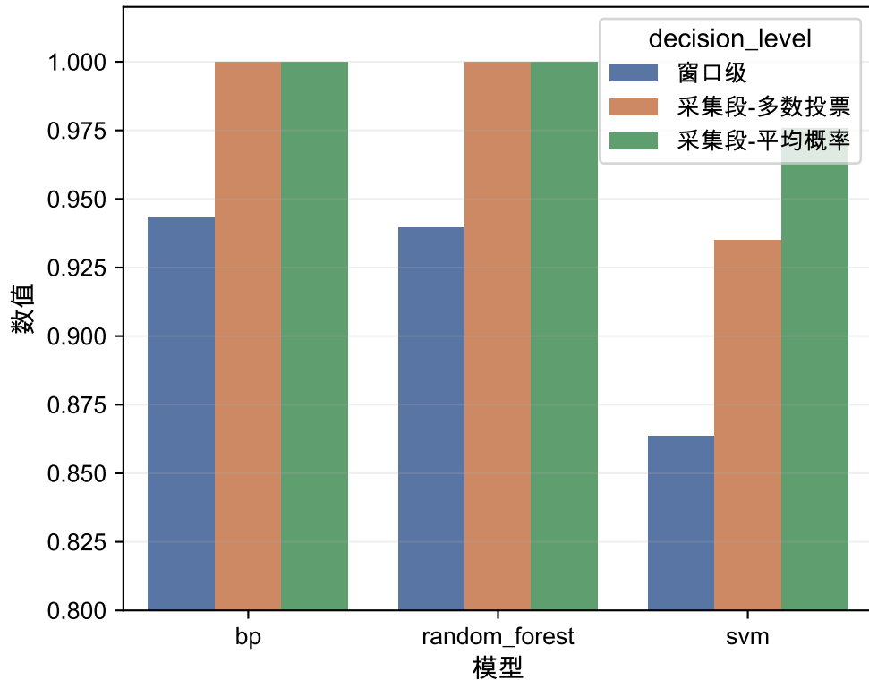
Accuracy 对比
