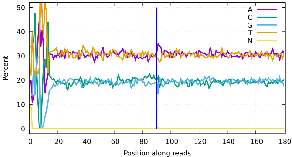
Base percentage composition along reads
