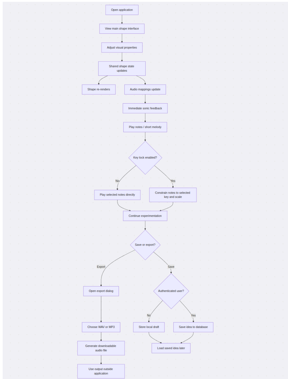
Figure 5: Main user flow
