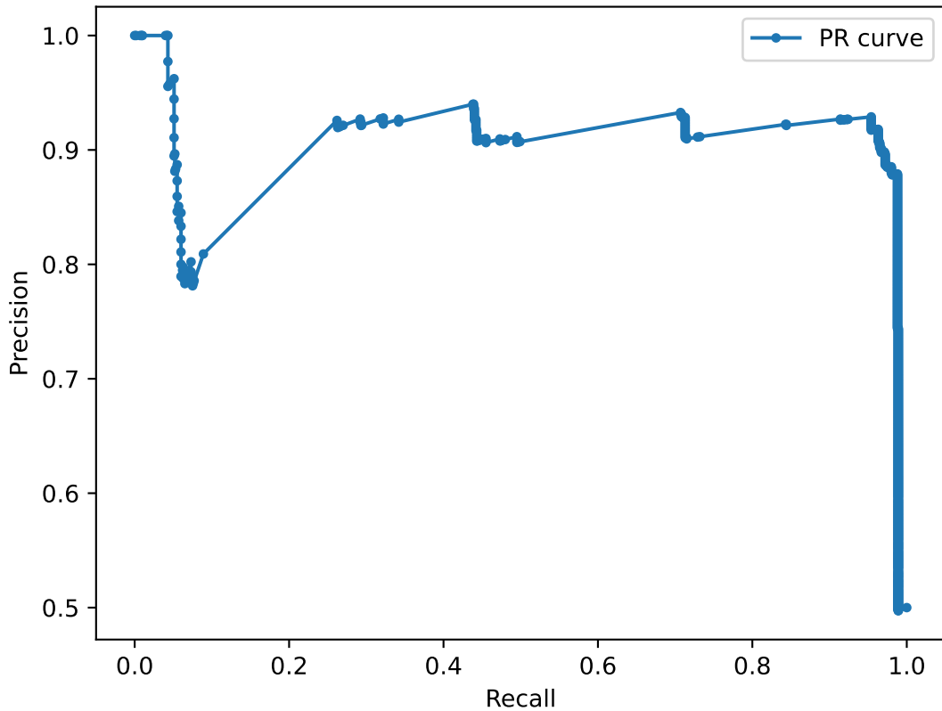
Precision Recall email-enron
