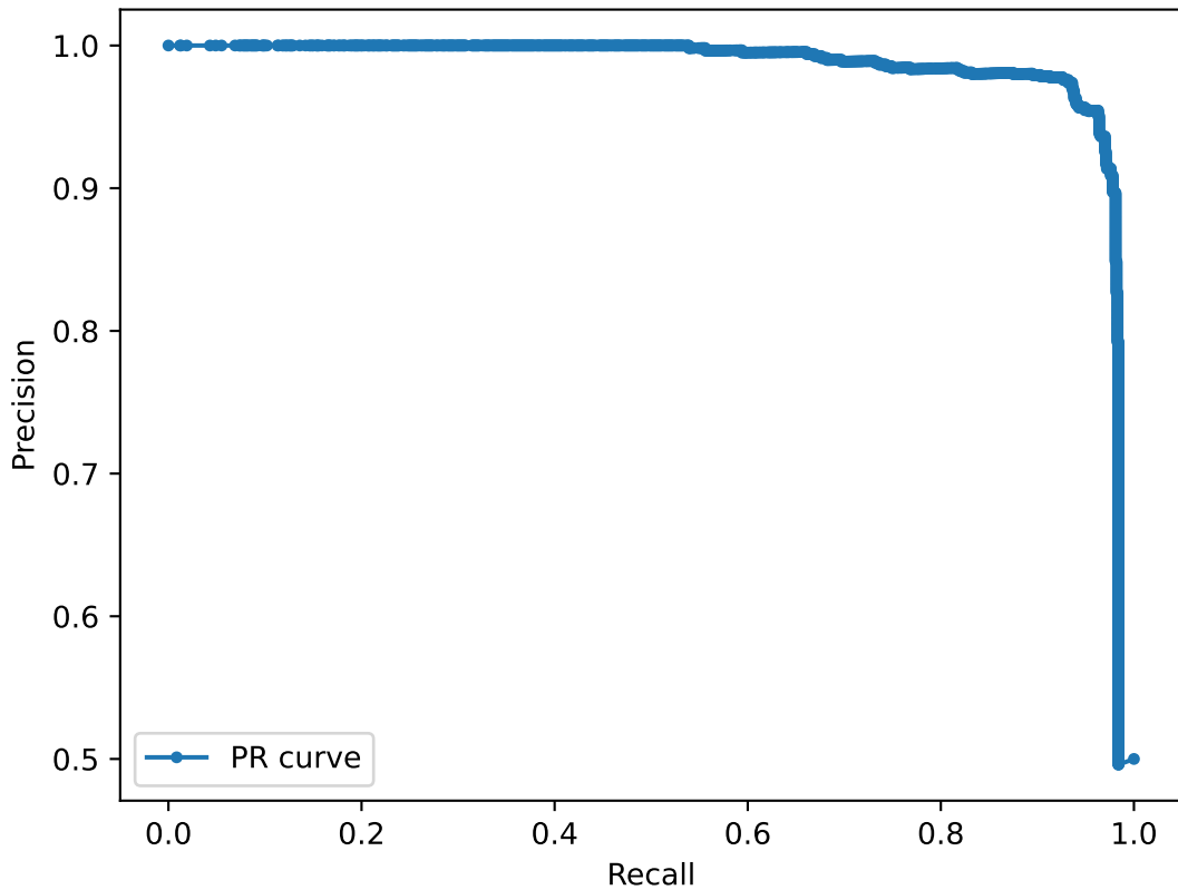
Precision Recall email-eu
