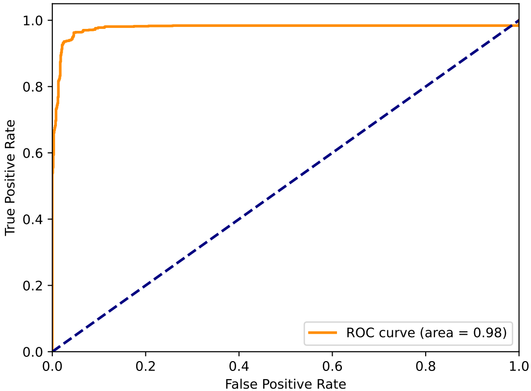
ROC curve email-eu
