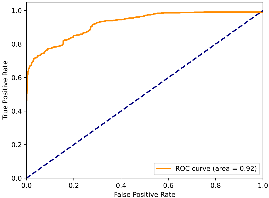
ROC curve tags-math-sx
