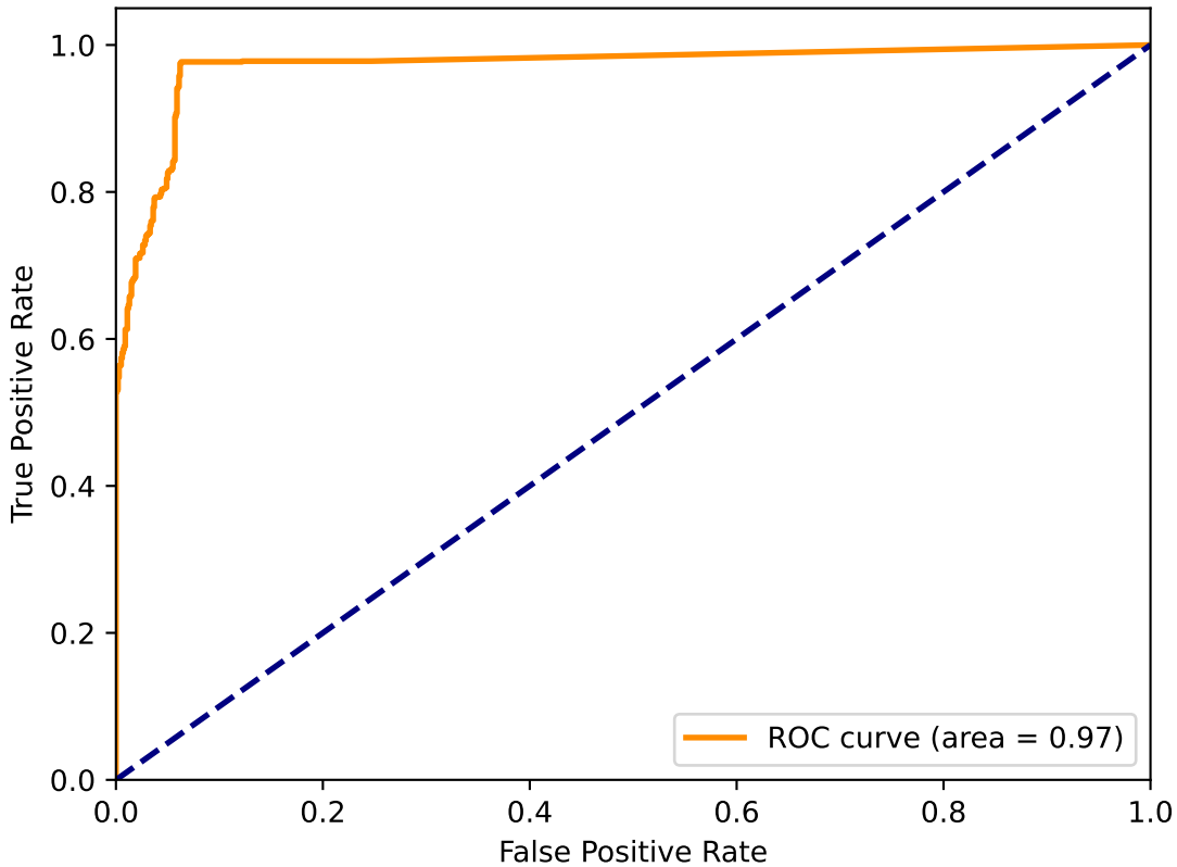
ROC curve congress-bills
