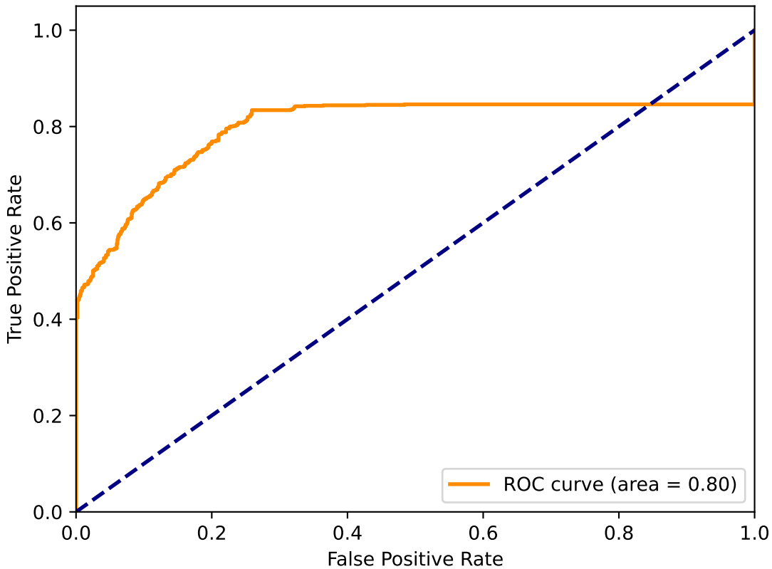
ROC curve contact-primary-school
