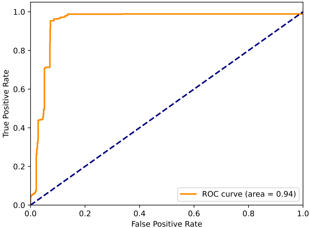
ROC curve email-enron
