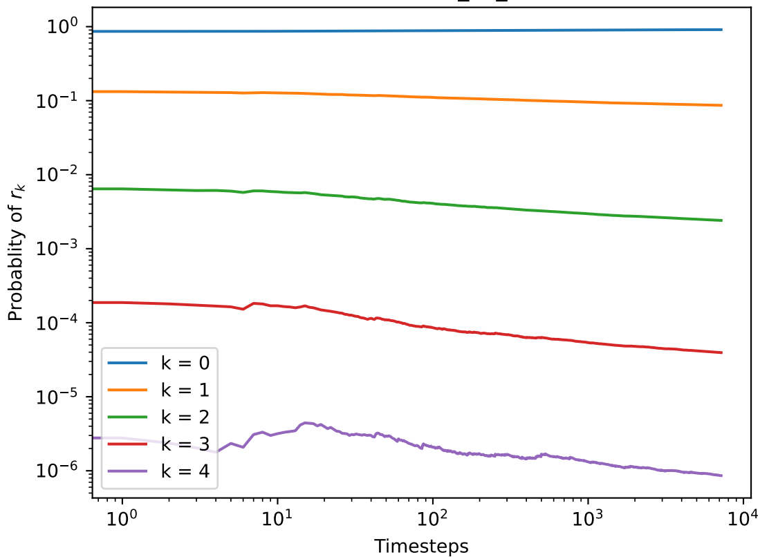
threads-math-sx_PA_exact
