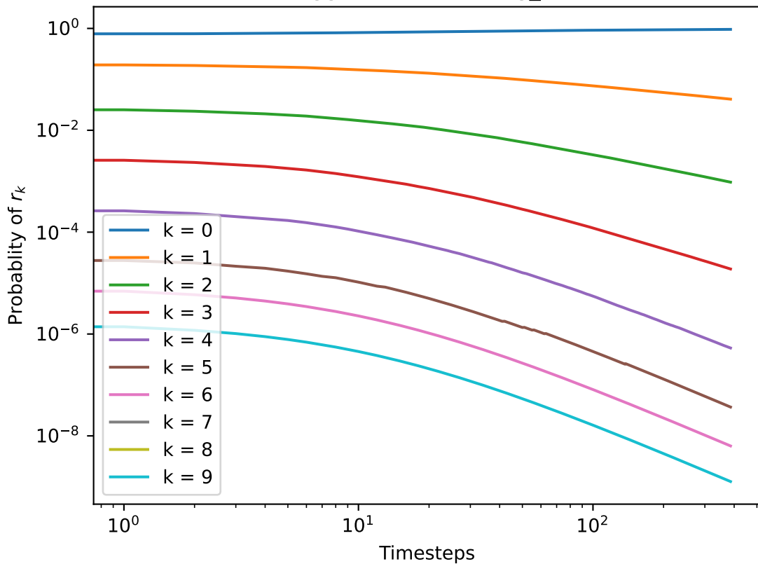
kaggle-whats-cooking_ER
