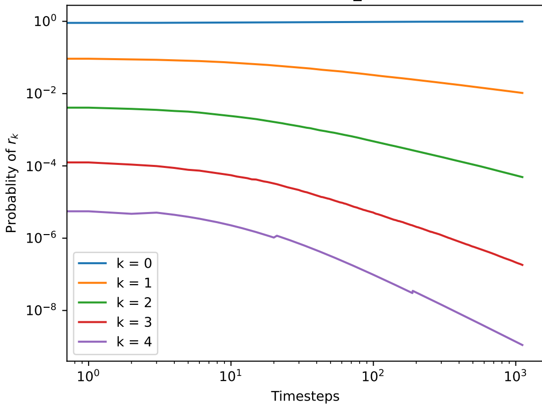
ndc-substances_ER
