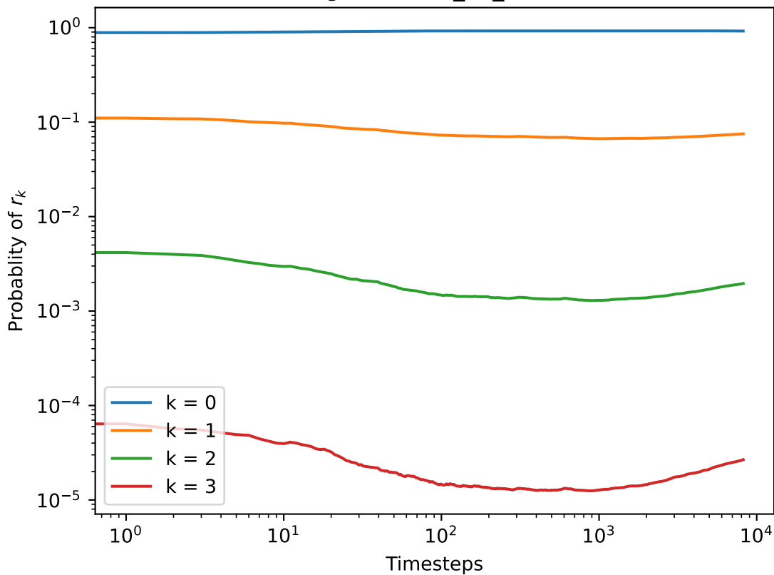
tags-math-sx_PA_exact
