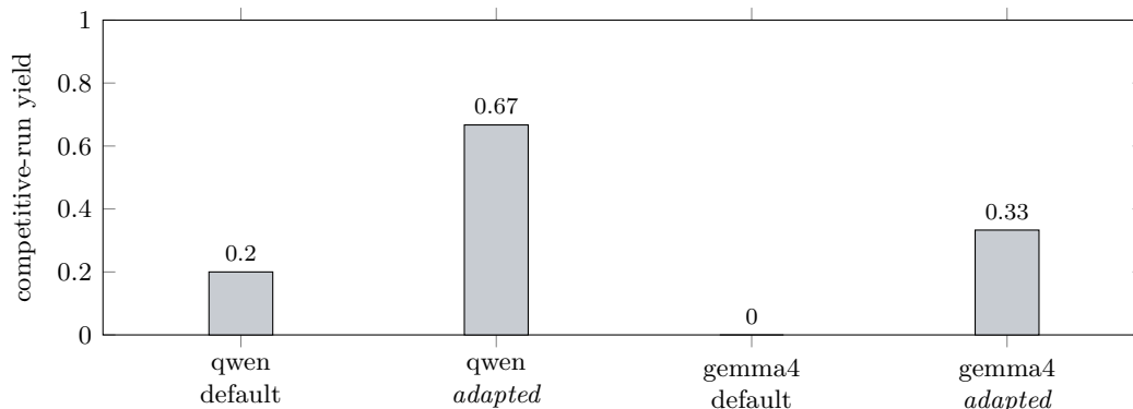
Figure 3: Companion observation (motivation, not a measured result of this paper). Fraction of SIA self-improvement runs that produced a competitive spaceship-titanic pipeline ( > 0.5 accuracy on held-out labels), by model and by target design. “Adapted” replaces SIA’s default nested-LLM-agent target — whose self-reports are unverified and which fails against the local endpoint’s stricter message validation — with a plain, directly-executed script that binds the model’s work to an external interpreter and grader. Counts: qwen-default 1/5, qwen-adapted 2/3, gemma-default 0/3, gemma-adapted 1/3. Yields are small- n and high-variance; the point is directional.
