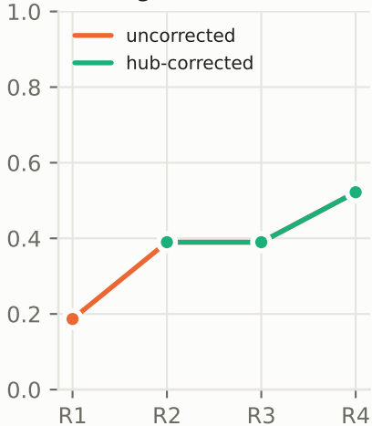
coverage C(30)
