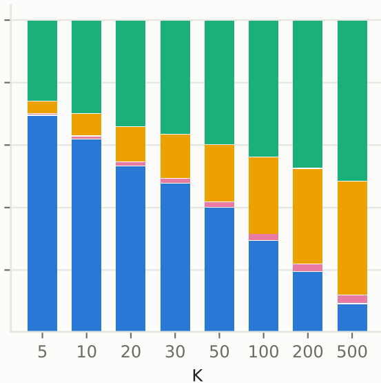
hub-corrected reranker
