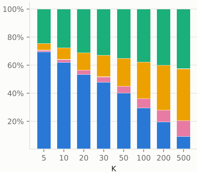
uncorrected reranker
