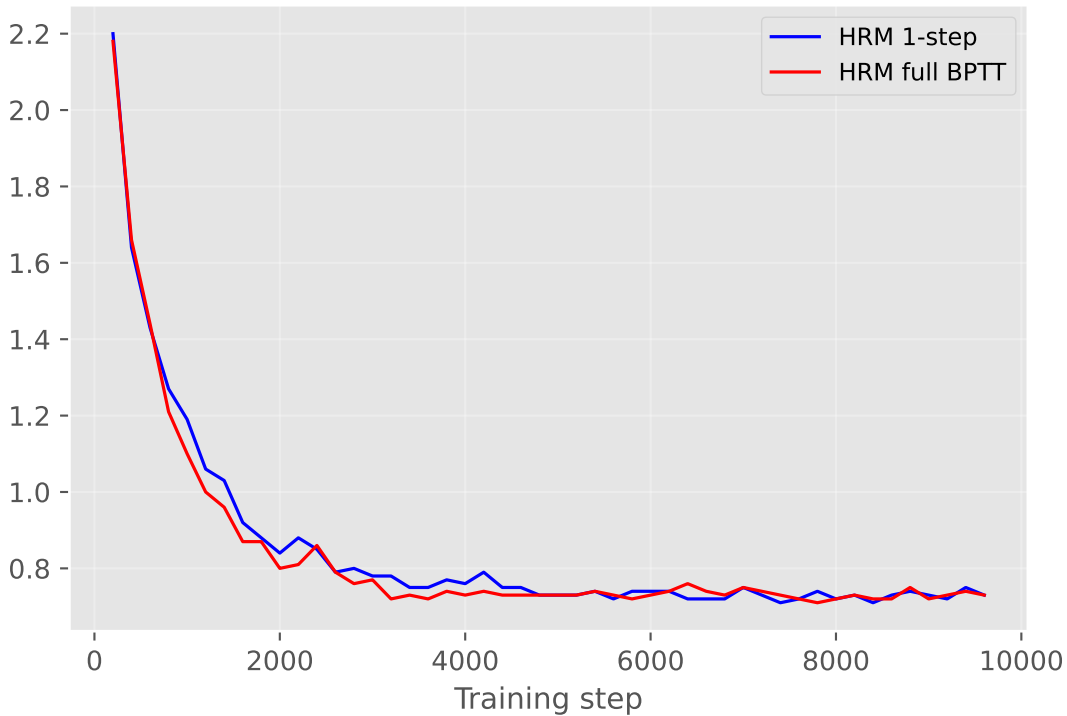
Stablemax cross-entropy loss
