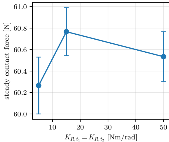
Rotational stiffness sweep
