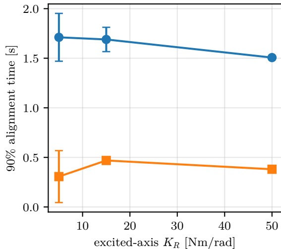
Case B: rotational stiffness
