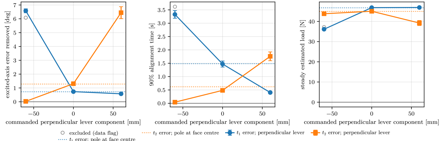
Case D: commanded centre of compliance, r_c = p_{\text{TCP}} - p_c
