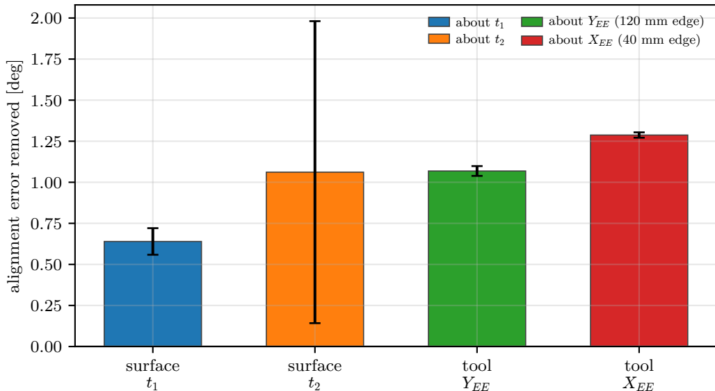
Case E: 10 deg tilt about surface vs tool axes
