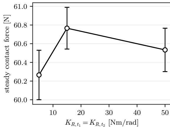
Rotational stiffness sweep
