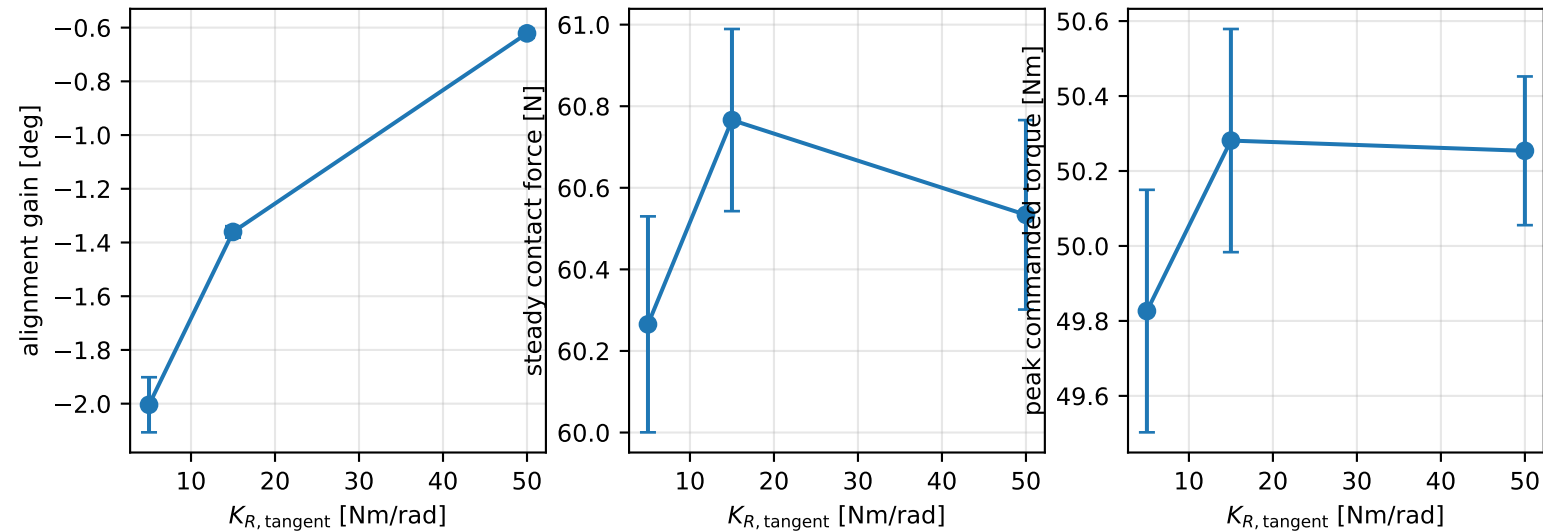
A2: rotational stiffness sweep (replaces thesis Table 5.1)
