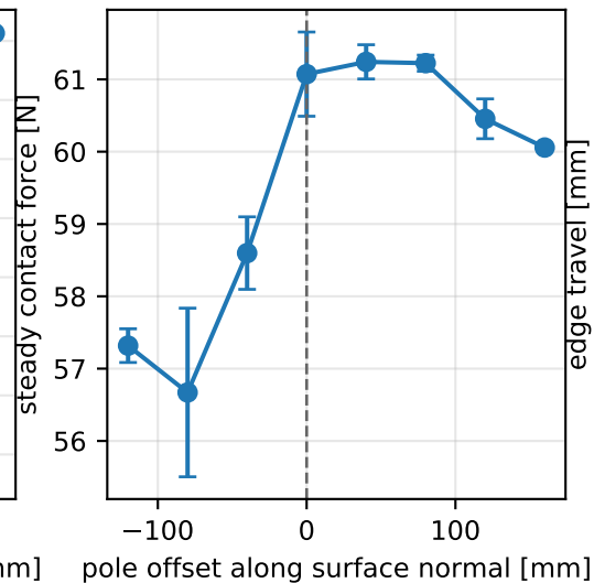
B2: pole swept along the surface normal
