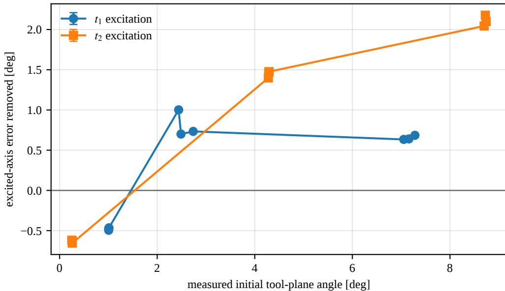
Case A: initial-angle response
