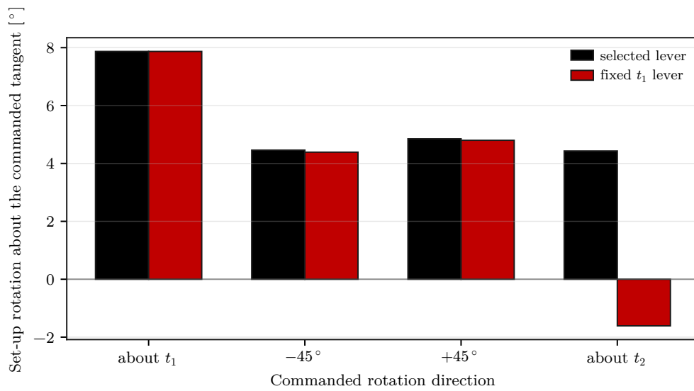
Figure 5.11: Case-C set-up rotation with the direction-selected and fixed levers.
