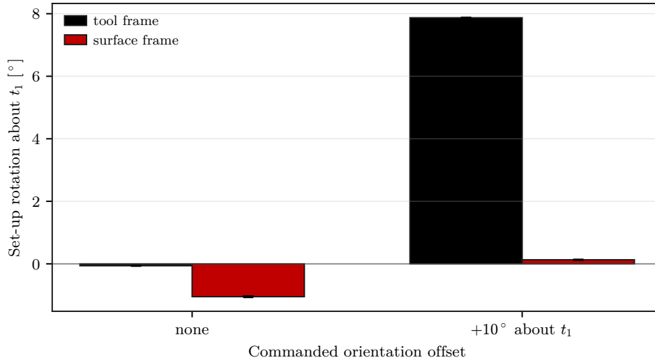
Figure 5.8: Case-F set-up rotation for tool- and surface-frame lever definitions.
