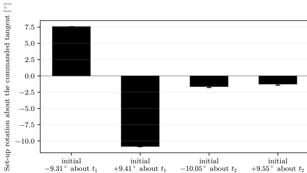
Figure 5.2: Set-up rotation with the centre of compliance at the TCP.
