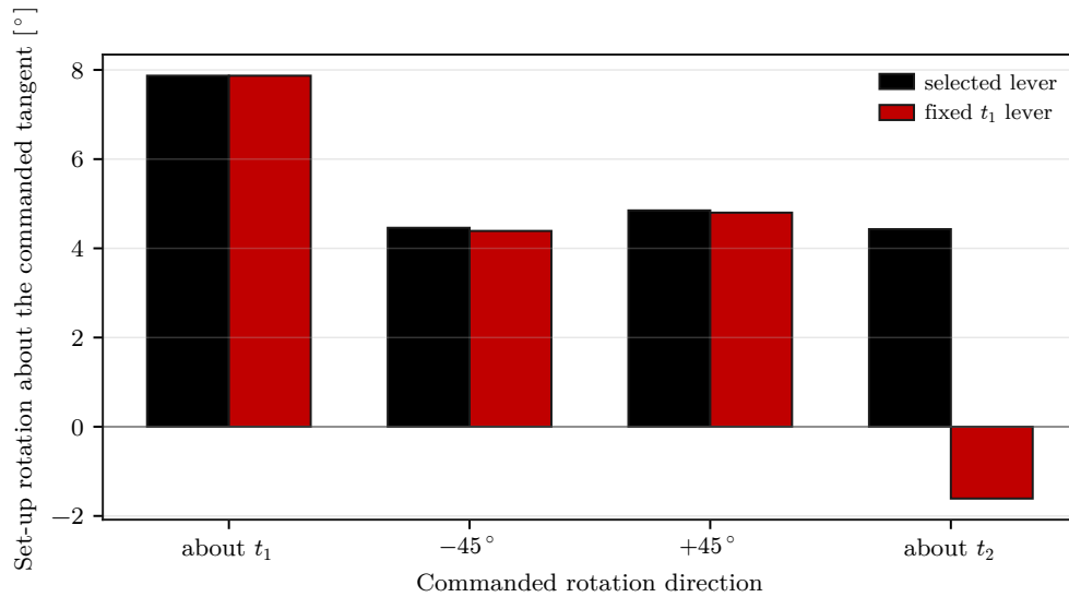
Figure 5.4: Case-C set-up rotation with the direction-selected and fixed levers.
