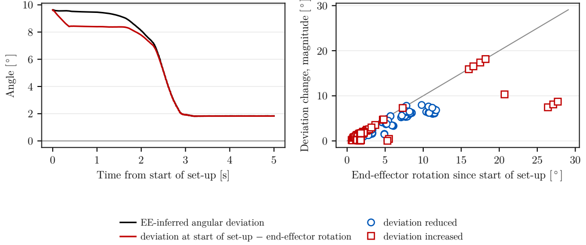
Figure 5.13: Agreement between the change in the EE-inferred angular deviation and the end-effector rotation since the start of set-up. The left panel overlays both quantities for one trial; the right panel compares their magnitudes for all archived trials.
