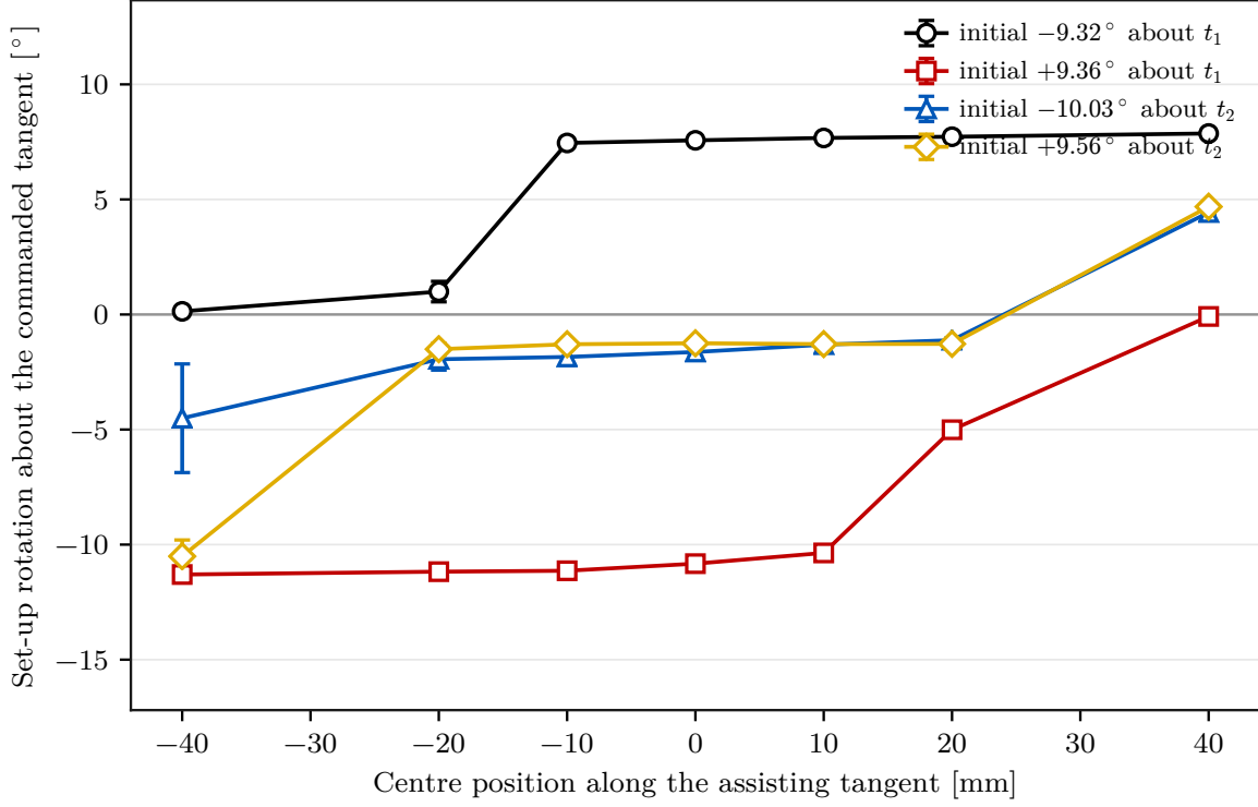
Figure 5.6: Signed set-up rotation about the commanded tangent by centre position, for both surface tangents and both signs of the commanded orientation offset.
