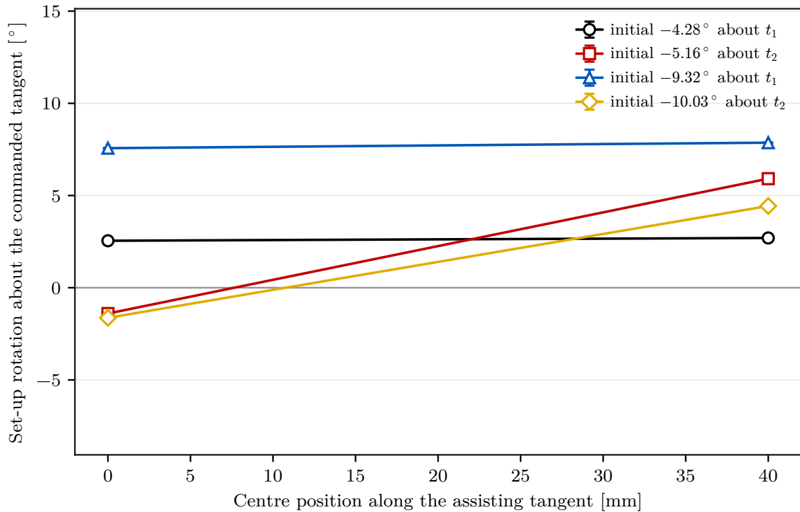
Figure 5.11: Signed set-up rotation about the commanded tangent at both commanded magnitudes, by centre position along the assisting tangent.
