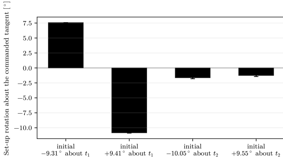
Figure 5.5: Signed set-up rotation about the commanded tangent with the centre of compliance on the TCP.
