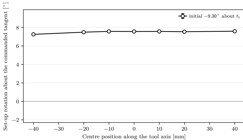
Figure 5.10: Signed set-up rotation about t_1 by centre position along the tool axis.
