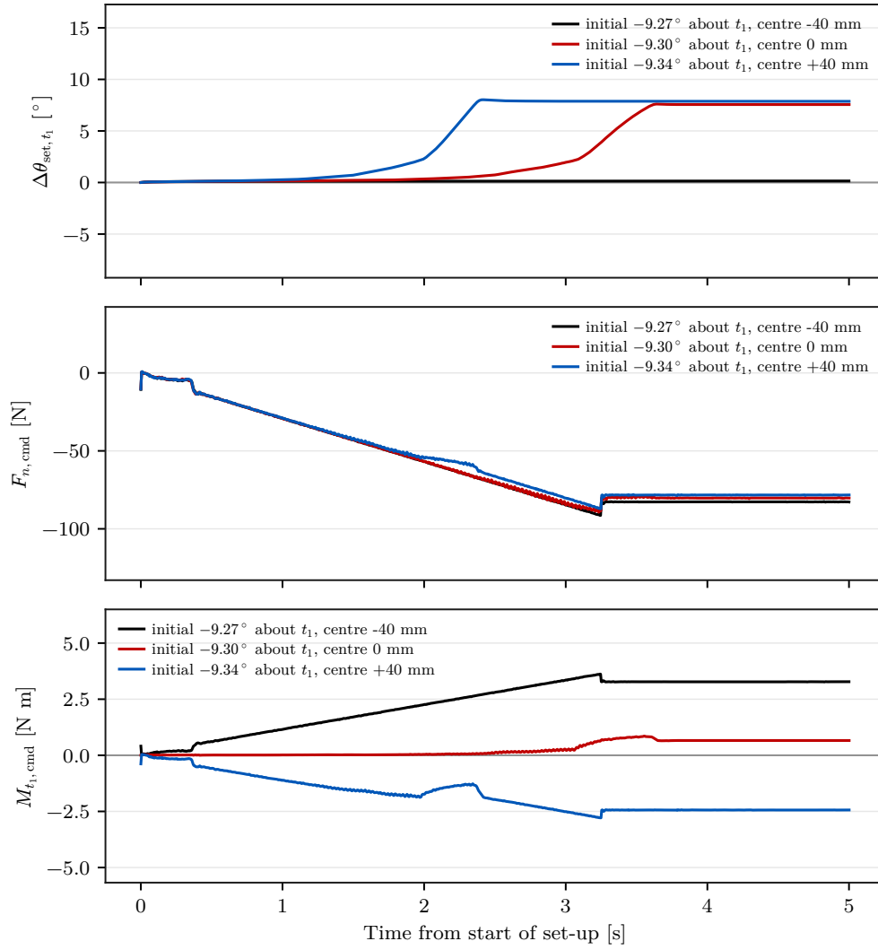
Figure 5.7: Set-up rotation \Delta\theta_{\text{set},t_1} , commanded normal force F_{n,\text{cmd}} , and commanded TCP moment M_{t_1,\text{cmd}} for three centre positions. All conditions carry a commanded orientation offset of +10^\circ about t_1 . The legends state the measured orientation at the beginning of set-up.
