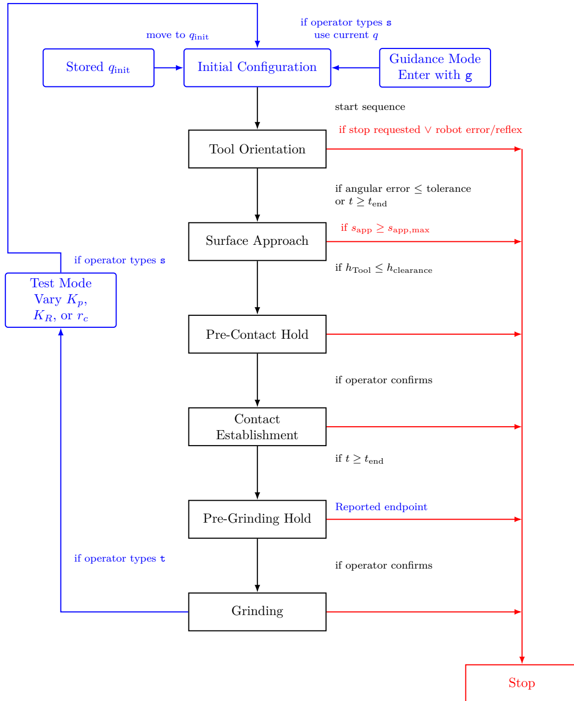
Figure 3.3: Surface-contact state transitions.
