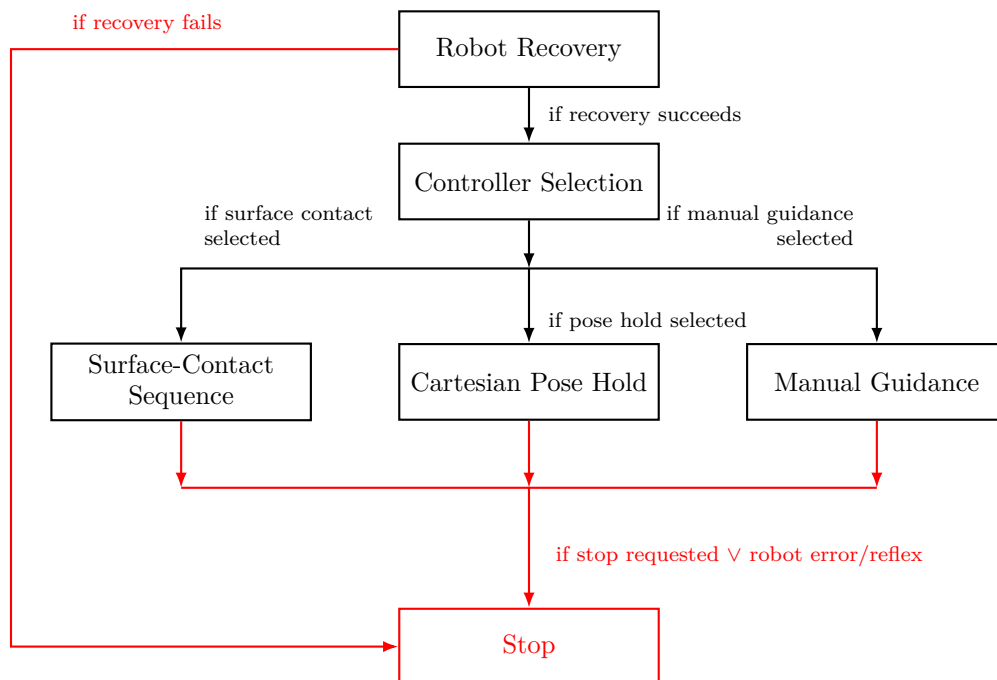
Figure 3.1: Controller operating-state flow.
