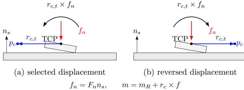
Figure 2.3: Normal-force contribution to the compliance-centre coupling moment for opposite tangential displacements: (a) the displacement selected from the angular-deviation direction; (b) the displacement with the opposite sign.
