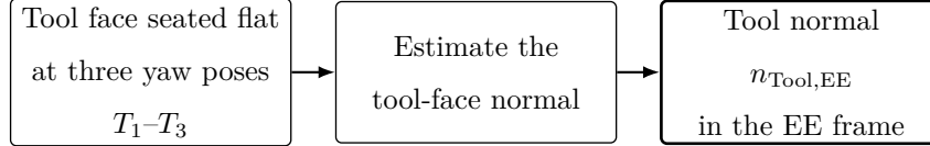
Figure 4.3: Surface-reference construction and tool-normal calibration.
