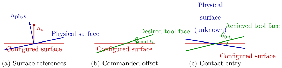
Figure 1.1: Configured surface reference, commanded tool offset, and contact-entry geometry. The physical normal is unknown to the controller, and the achieved reference-relative angle need not equal the command. +
