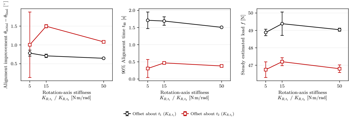
Figure 5.2: Case-B alignment improvement by rotation-axis stiffness.
