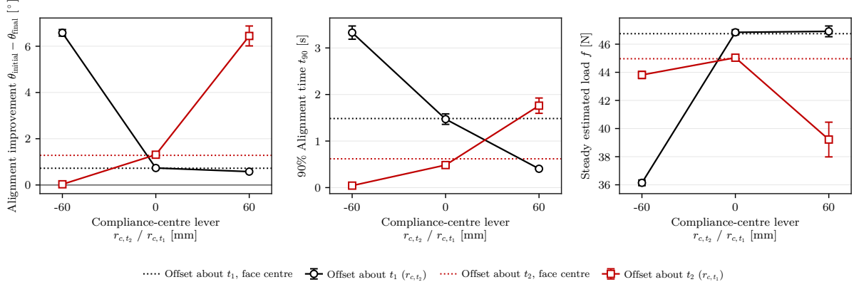
Figure 5.4: Case-D alignment response for the tested compliance-centre levers.
