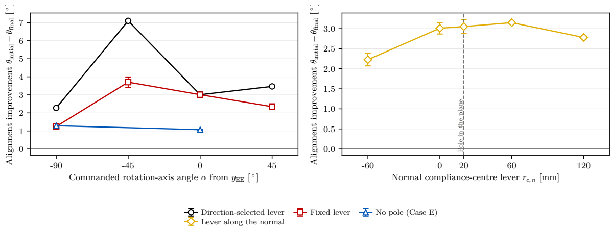
Figure 5.9: Alignment response by rotation direction and normal lever coordinate.
