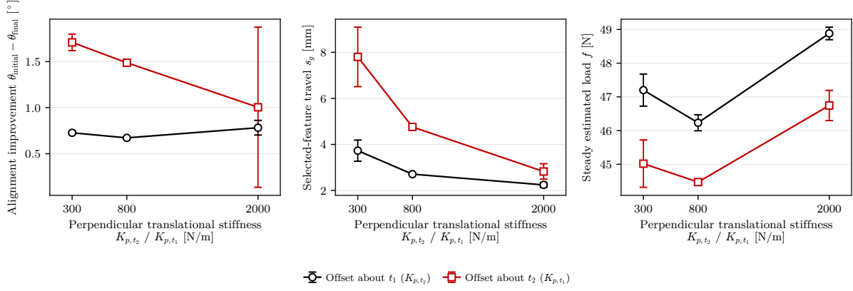
Figure 5.3: Case-C alignment improvement for the tested perpendicular translational stiffnesses.
