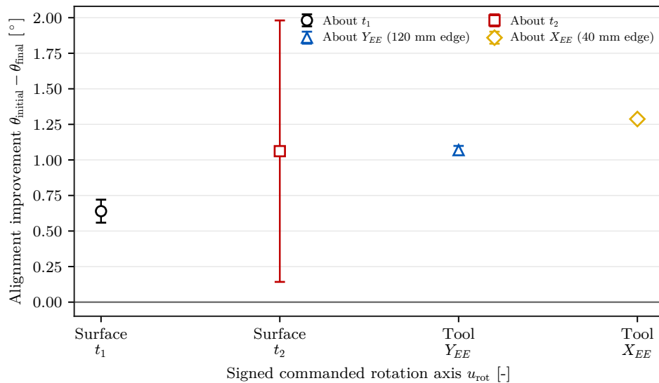
Figure 5.5: Case-E alignment improvement by commanded rotation axis.
