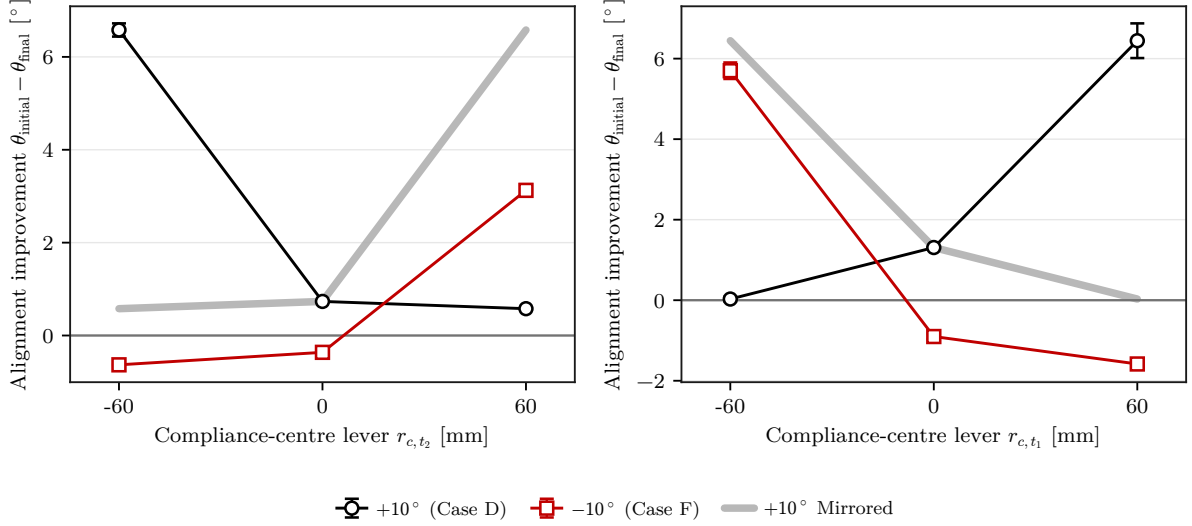
Figure 5.6: Alignment improvement by offset direction and compliance-centre lever.
