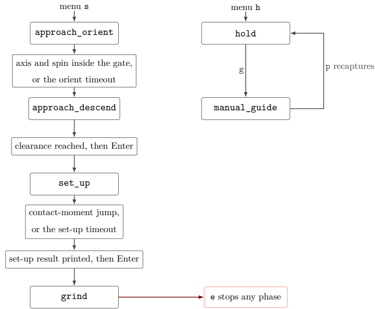
Figure 3.2: Run phase sequence and Cartesian pose hold.
