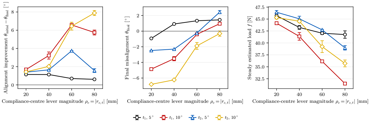
Figure 5.8: Alignment improvement, residual angle, and load by lever magnitude.
