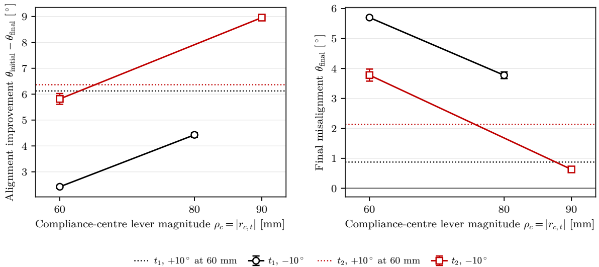
Figure 5.7: Reversed-offset response at the extended lever magnitudes.
