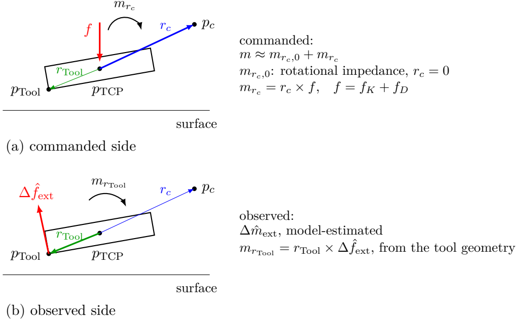
Figure 2.2: Commanded and observed moment relations: (a) the translation-induced coupling carried by the commanded wrench; (b) the model-estimated external interaction with the geometry-based force-lever moment.
