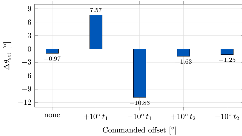
Figure 5.1: Set-up rotation with the centre of compliance at the TCP.
