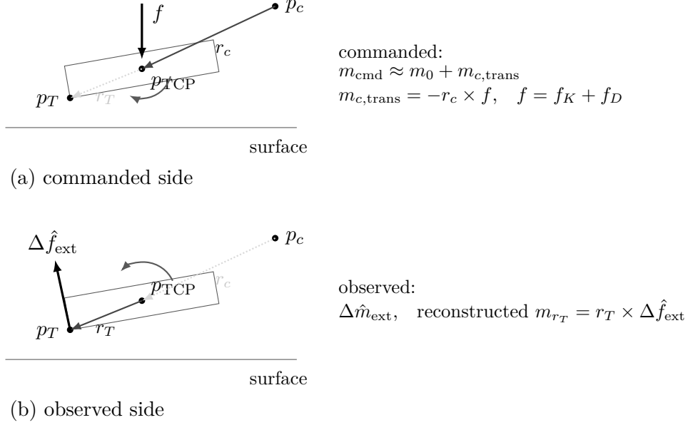
Figure 2.2: Moment relations on the commanded and observed sides.
