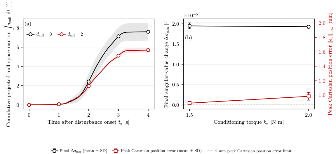
Figure 5.10: Null-space response during the Cartesian pose-hold disturbance test. In (a), the solid curves show the mean cumulative projected null-space motion and the shaded bands indicate \pm one standard deviation across the three repetitions.
