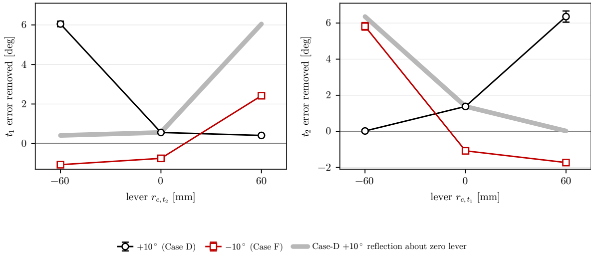
Figure 5.6: Alignment improvement at both tilt signs, by compliance-centre lever.
