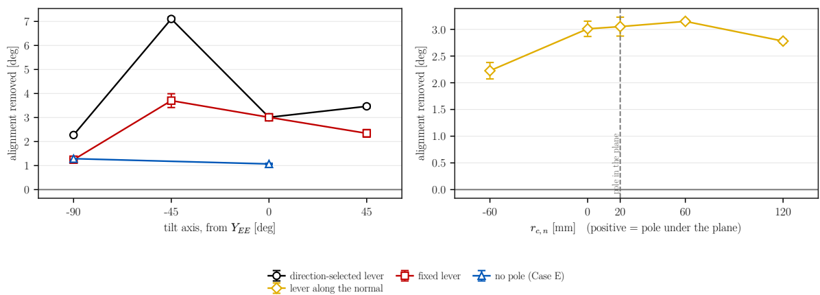
Figure 5.9: Alignment response by tilt direction and by normal lever coordinate.
