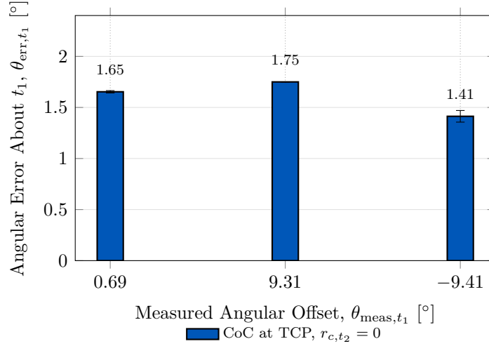
Figure 5.4: Angular error with the CoC at the TCP.
