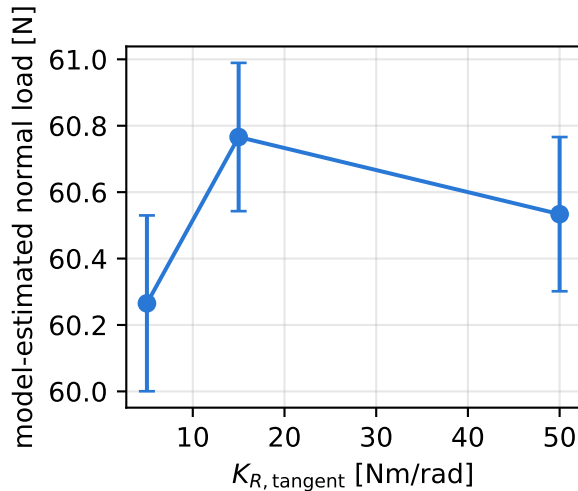
Influence of tangential rotational stiffness
