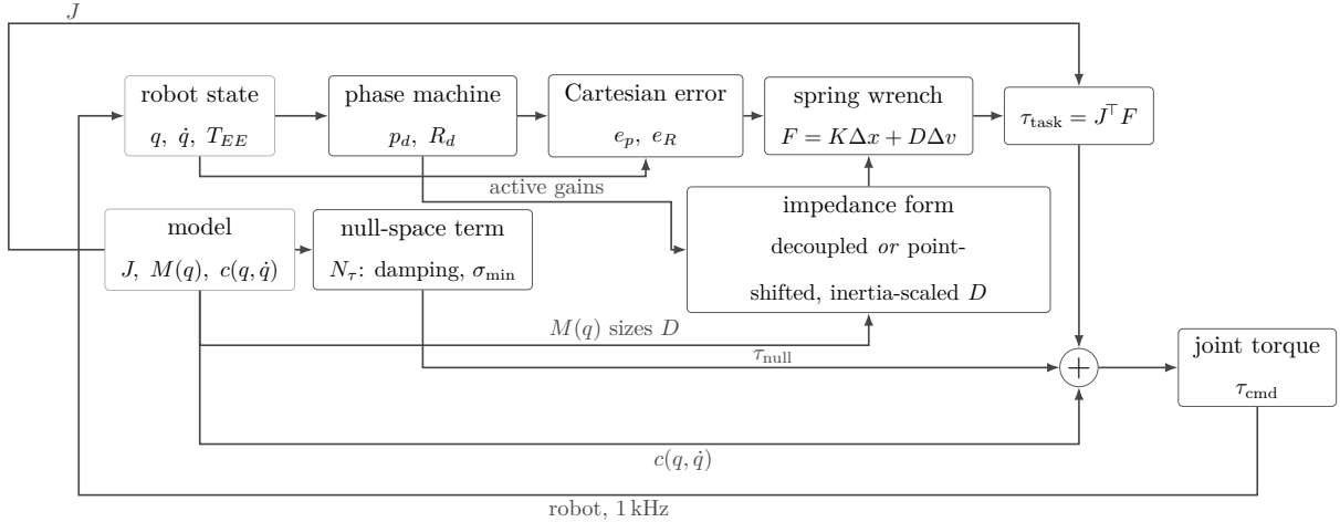
Figure 3.1: Torque contributions combined in one control cycle.
