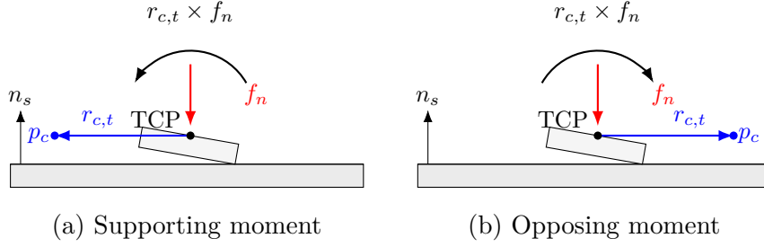
Figure 2.3: Normal-force contribution for (a) the selected tangential displacement and (b) its reversal.
