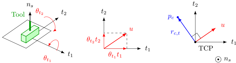
(a) Tangent rotations (b) First-order direction (c) Selected displacement
