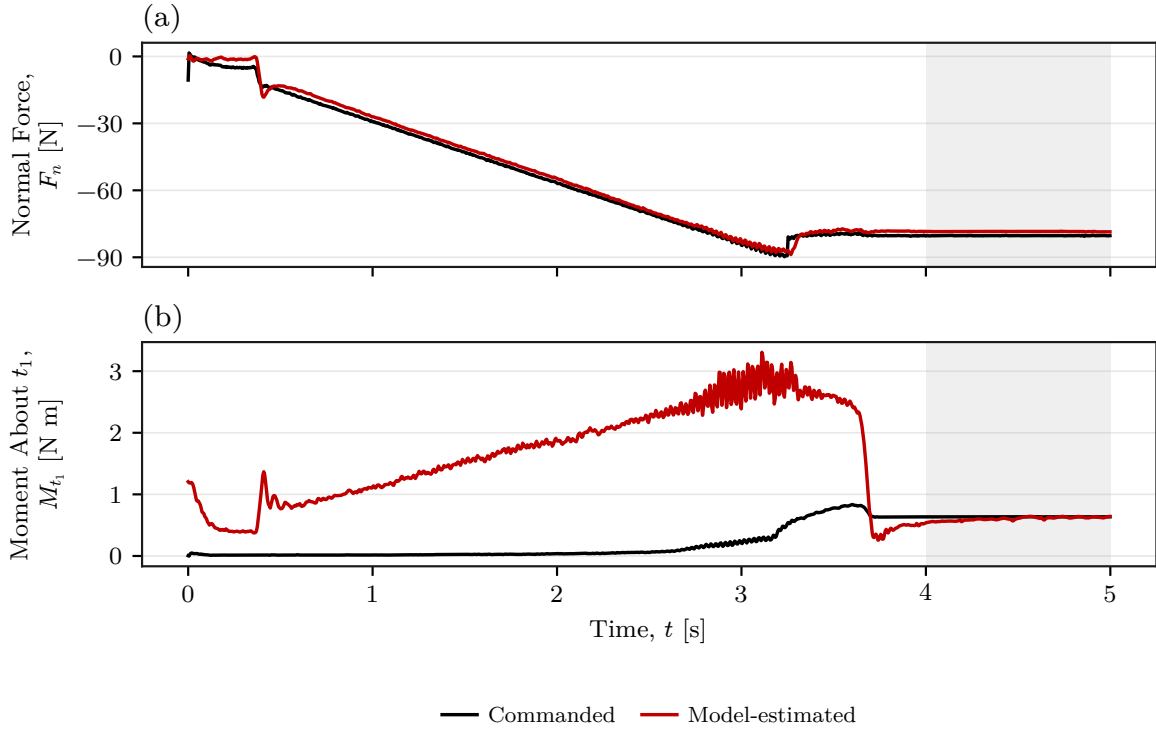
Figure 5.1: Commanded and model-estimated wrench during Contact Establishment.
