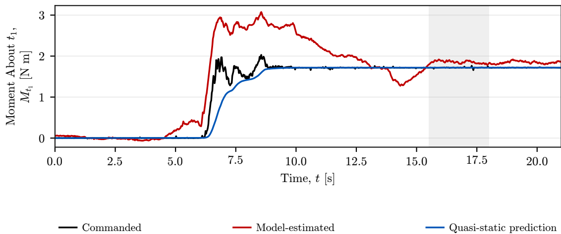
Figure 5.3: Quasi-static moment plausibility assessment about the first surface tangent.
