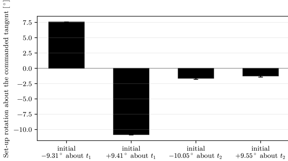
Figure 5.2: Set-up rotation with the centre of compliance at the TCP.
