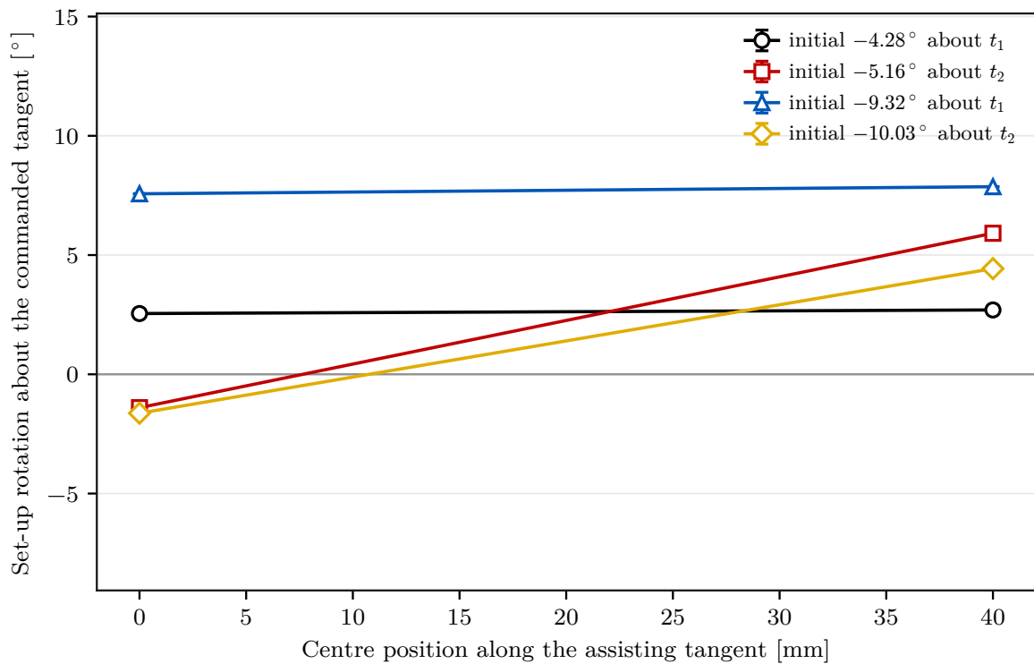
Figure 5.10: Set-up rotation by centre position at both commanded magnitudes.
