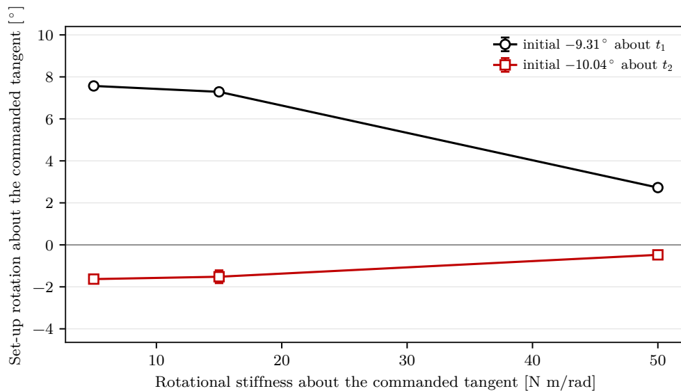
Figure 5.3: Set-up rotation about the commanded tangent by rotational stiffness.
