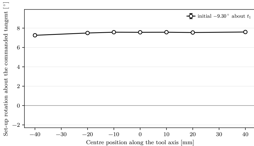
Figure 5.9: Set-up rotation by centre position along the tool axis.
