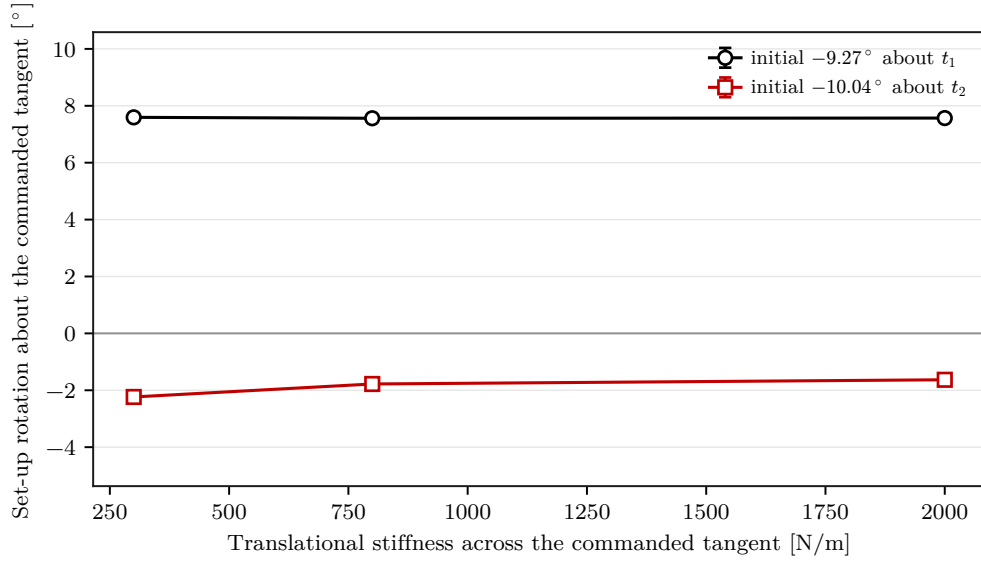
Figure 5.4: Set-up rotation by cross-axis translational stiffness.
