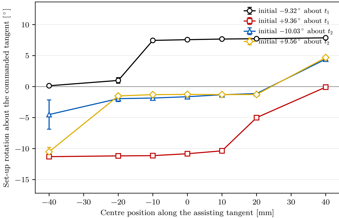
Figure 5.5: Set-up rotation by tangential centre position, both tangents and signs.
