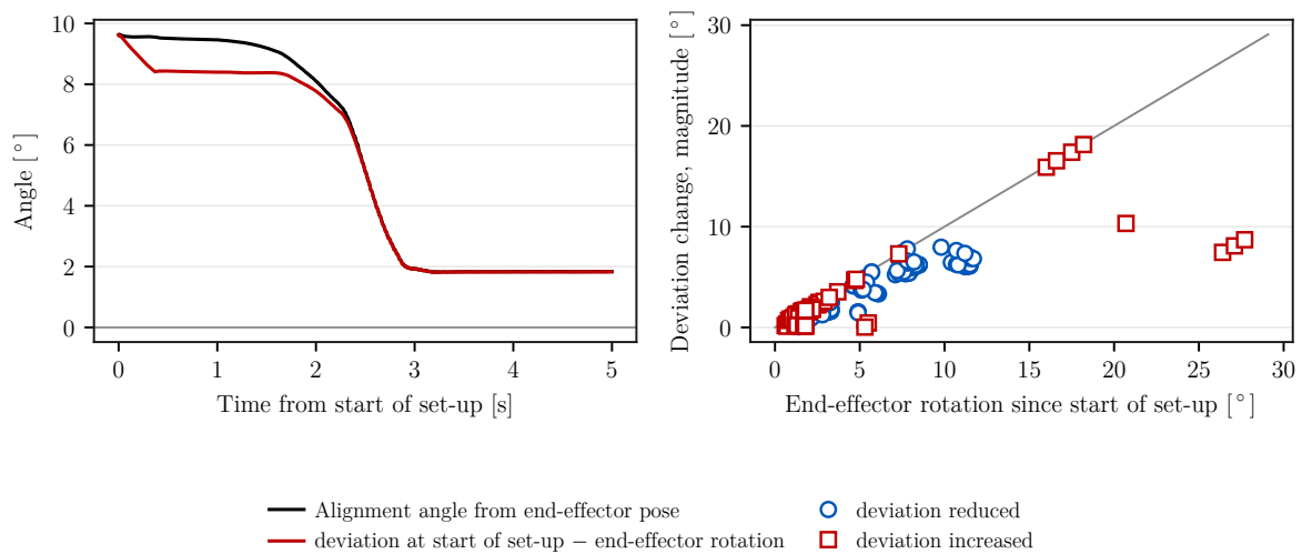
Figure 5.13: Comparison between the change in the alignment angle calculated from the end-effector pose and the end-effector rotation since the start of set-up. The left panel shows both quantities for one representative trial. The right panel compares their magnitudes over all archived trials and distinguishes whether the calculated alignment angle decreased or increased during set-up.
