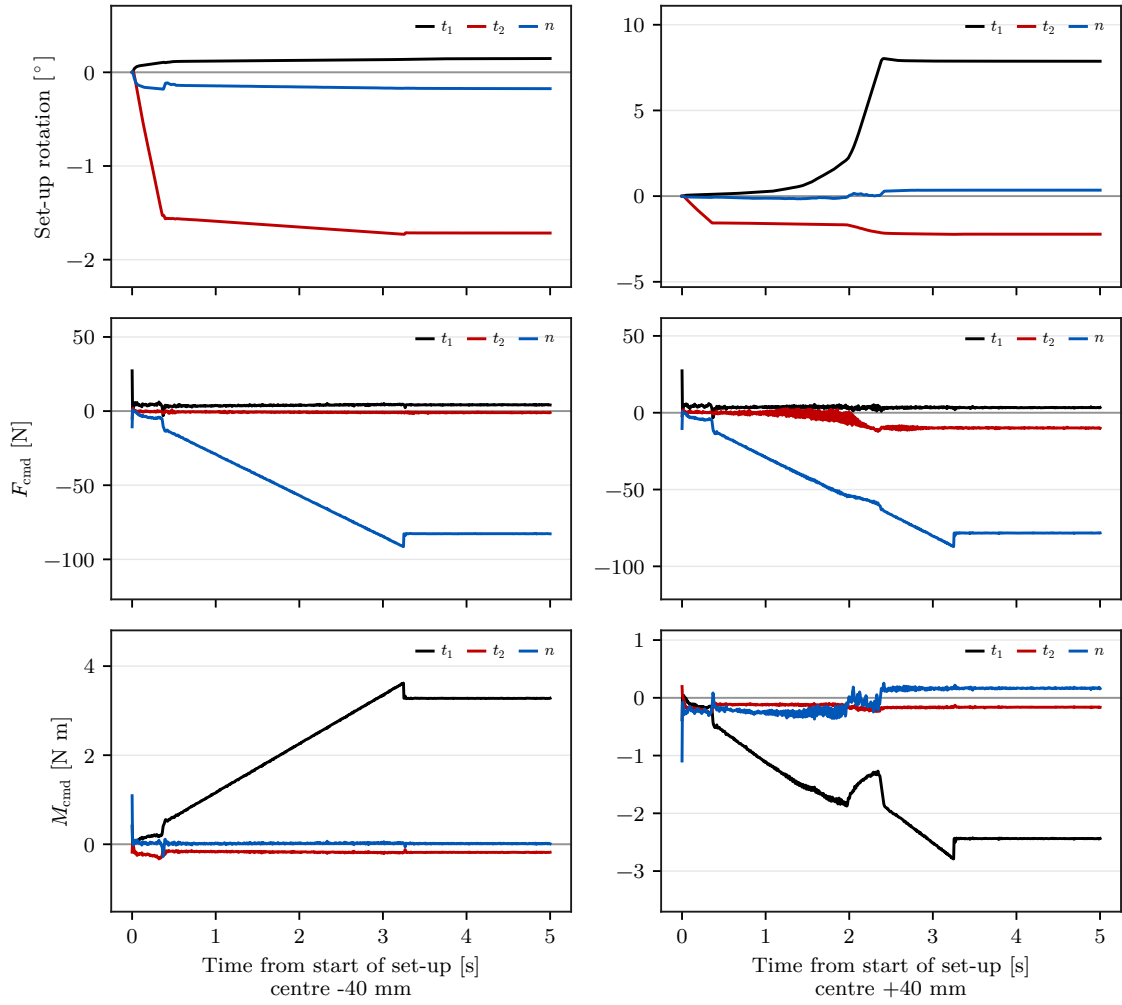
Figure 5.7: Surface-frame rotation, force and moment at the outer Case-D positions.
