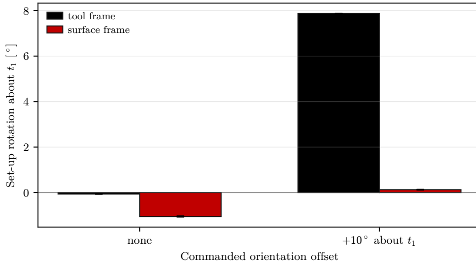
Figure 5.8: Case-E set-up rotation for tool- and surface-frame lever definitions.
