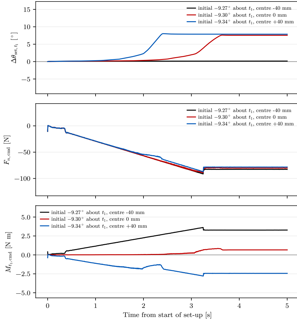
Figure 5.6: Set-up rotation \Delta\theta_{\text{set}, t_1} , commanded normal force F_{n, \text{cmd}} , and commanded TCP moment M_{t_1, \text{cmd}} for three centre positions. All conditions carry a commanded orientation offset of +10^\circ about t_1 . The legends state the measured orientation at the beginning of set-up.
